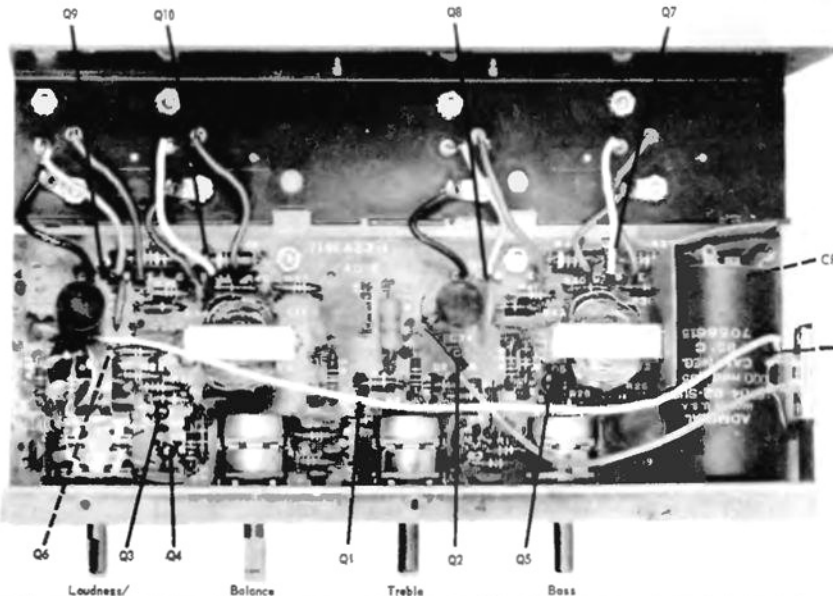
TOP VIEW OF CHASSIS OPENED FOR SERVICING
